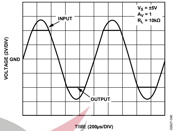
Figure 40. No Phase Reversal
