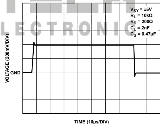
Figure 57. Capacitive Load Drive with Snubber
