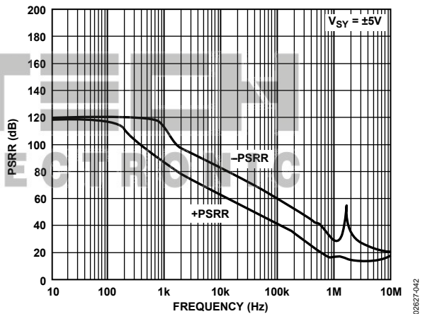
Figure 42. PSRR vs. Frequency
