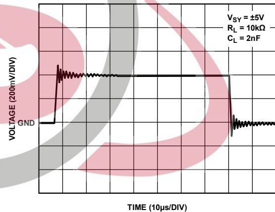
Figure 56. Capacitive Load Drive Without Snubber
