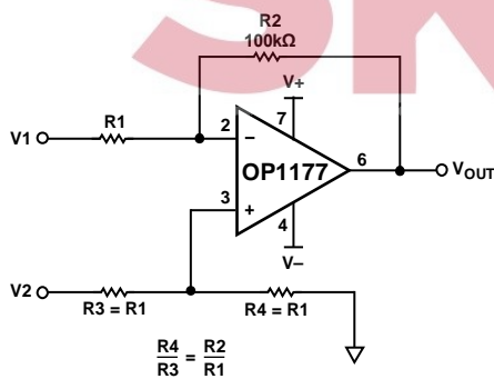
Figure 63. Difference Amplifier
