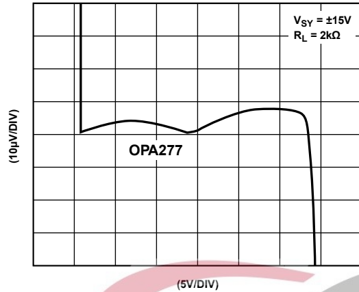
Figure 52. Gain Linearity
